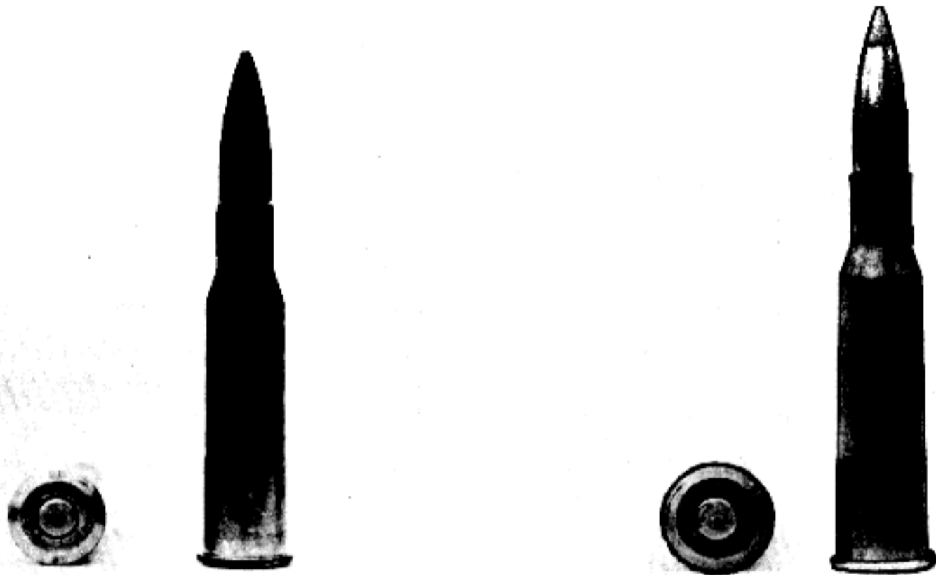
FIGURE 33. SOVIET RIFLE AMMUNITION (LIGHT BALL ON LEFT, HEAVY BALL ON RIGHT).
